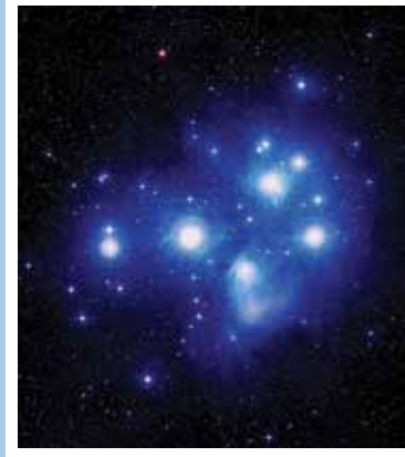
Pleiades star cluster
