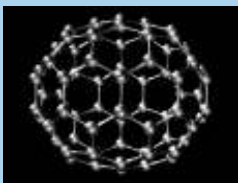
Allotrope
